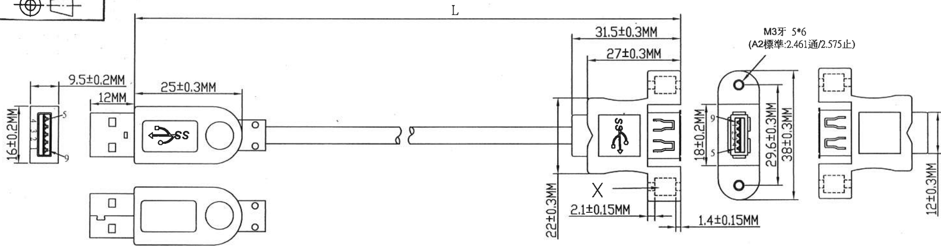
USB 3.0 AM(NICKEL PLATED) BLUE MOLDING(45P)
